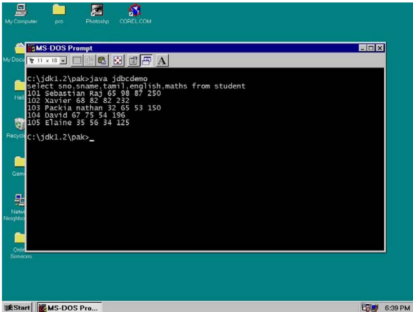
Listing 6.7
